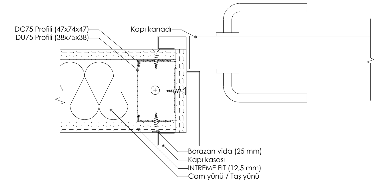
DETAY 09: TEK İSKELET SİSTEMİ KAPI PLANI (VİDALAMA)
