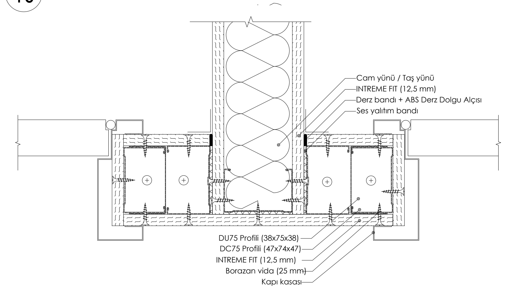
DETAY 10: TEK İSKELET SİSTEMİ KAPI PLANI (VİDALAMA)
