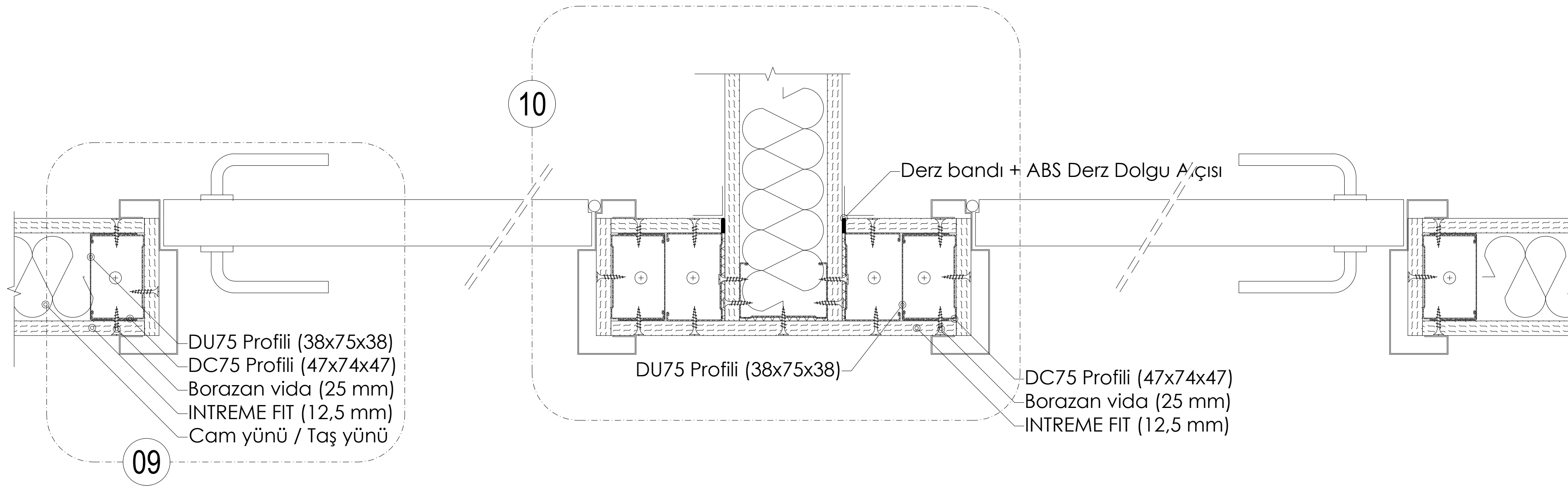
PLAN: TEK İSKELET SİSTEMİ KAPI DETAYI (VİDALAMA)
