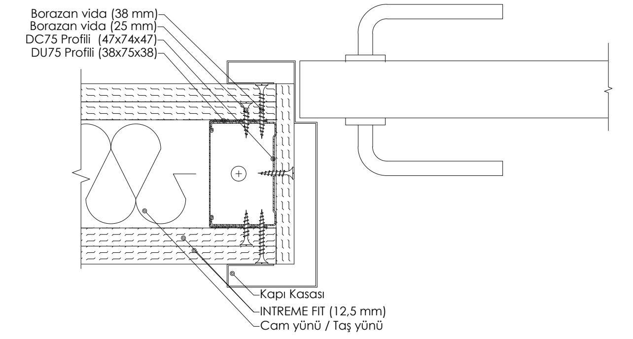
DETAY 09: TEK İSKELET SİSTEMİ KAPI PLANI (VİDALAMA)
