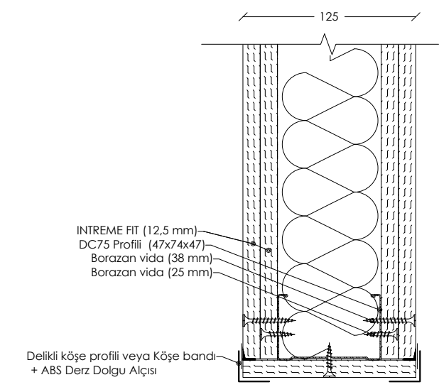
DETAY 07: TEK İSKELET SİSTEMİ DİŞ DUVAR PLANI
