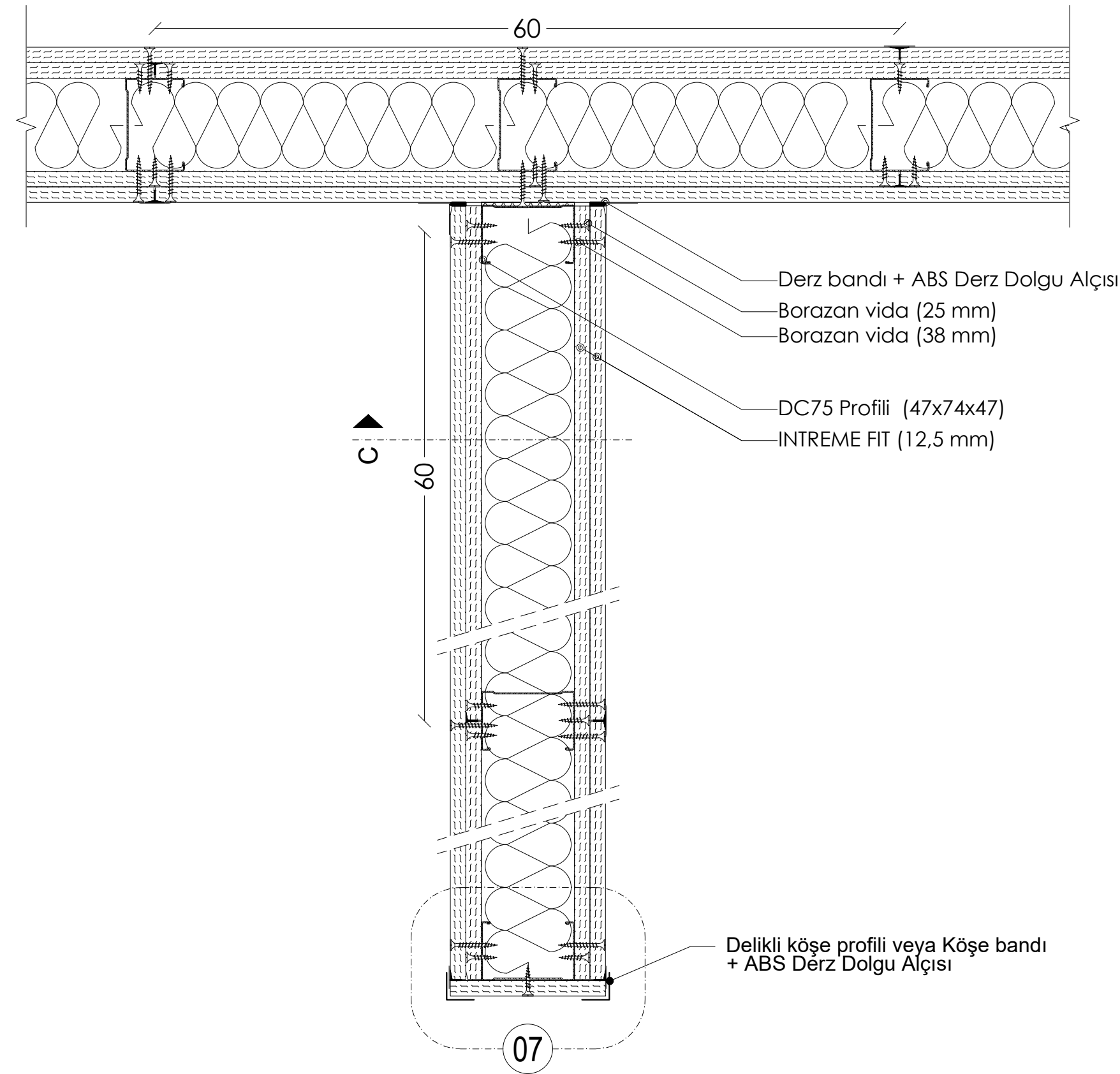
PLAN: TEK İSKELET SİSTEMİ DİŞ DUVAR
