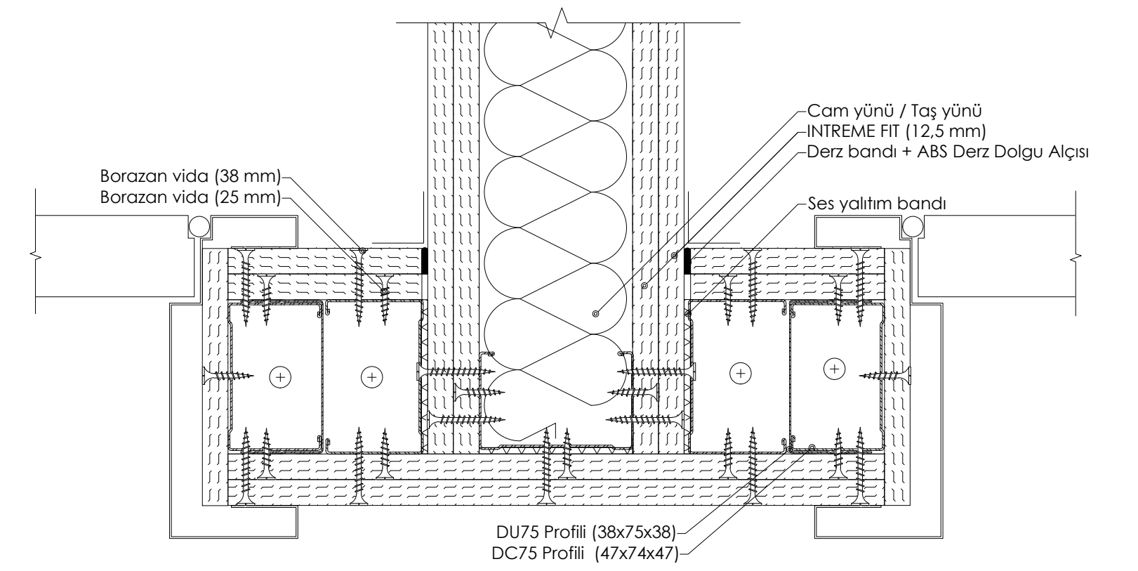
DETAY 10: TEK İSKELET SİSTEMİ KAPI PLANI (VİDALAMA)
