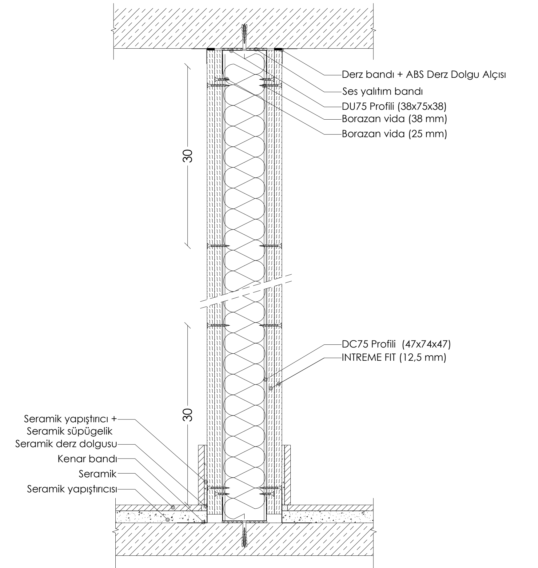
KESİT C: TEK İSKELET SİSTEMİ SERAMİK ZEMİN
